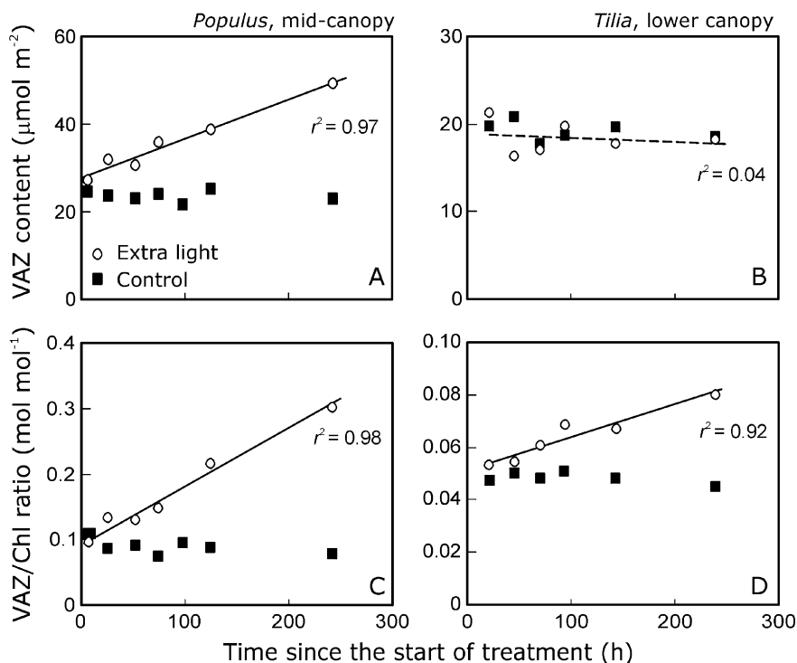
Fig. 5 Changes in xanthophyll cycle carotenoid content per unit area (A, B) and chlorophyll (C, D) due to extra light of 500–700 μmol m -2 s -1 for 12 h photoperiod in Populus tremula and Tilia cordata . Recalculated from Niinemets et al. (2003 a). Data were fitted by linear regressions. The regressions depicted with the solid line are significant at p < 0.001 .
