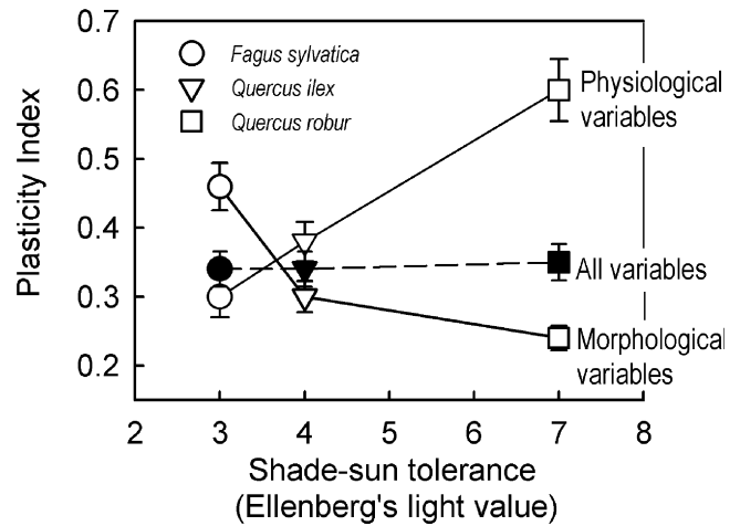
Fig. 3 Plastic response to light availability of seedlings of three widespread European tree species ( Fagus sylvatica – circles, Q. ilex – triangles, and Quercus robur – squares) differing in shade tolerance. Lower value of Ellenberg's light index indicates higher shade tolerance (Ellenberg et al., 1991). Values of the plasticity index were calculated for all variables pooled (six variables; solid symbols), and separately for three physiological (photosynthetic capacity, maximum stomatal conductance, and Rubisco activity) and three morphological variables (root-to-shoot ratio, leaf size, and leaf mass ratio; open symbols). Error bars give \pm SE. Elaborated from Valladares et al. (2002a, b).
