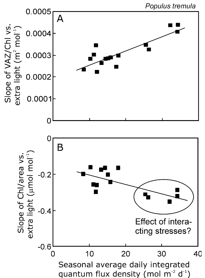
Fig. 7 Influences of integrated irradiance on (A) the slope of the VAZ/Chl versus cumulative extra light, and (B) the slope of leaf chlorophyll content versus cumulative extra light in Populus tremula (modified from Niinemets et al., 2003a). Extra light of 500\text{--}700 \mu\text{mol m}^{-2} \text{ s}^{-1} was applied during a 12 h photoperiod for 11 days (Fig. 5), and the time-dependent increases in VAZ/Chl and Chl/area were fitted by linear regressions for every leaf developed under the specific irradiance environment. Data points in A and B were fitted by linear regressions. The relationships depicted were significant at p < 0.001 (A) and p < 0.05 (B).
